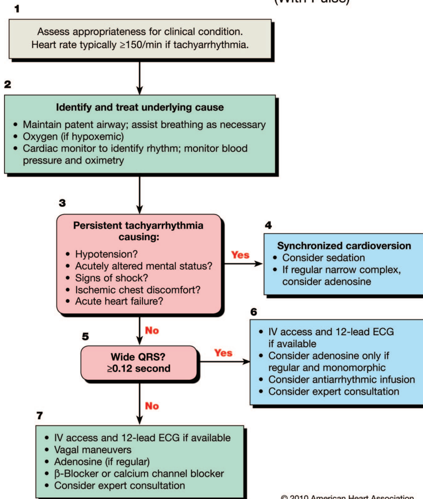
Figure 4. Tachycardia Algorithm.
